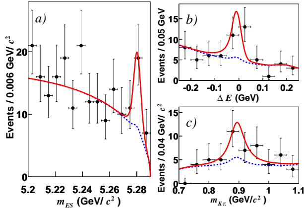
Figure 11. Evidence for B \rightarrow K^*\ell^+\ell^- from BaBar.
