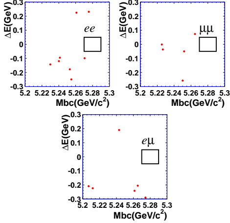
Figure 20. B_d^0 \rightarrow \ell^+ \ell^- search results from Belle.
