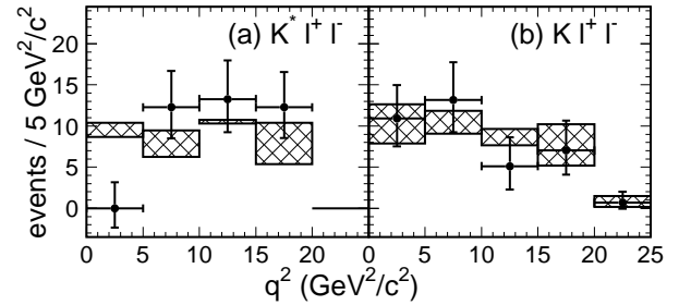
Figure 13. q^2 distributions for B \rightarrow K^{(*)}\ell^+\ell^- from Belle.
