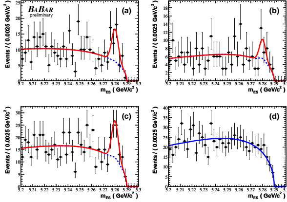
Figure 15. (a) B \rightarrow X_s e^+ e^- , (b) B \rightarrow X_s \mu^+ \mu^- , (c) B \rightarrow X_s e^+ \mu^- signals with the (d) X_s e^+ \mu^- sample from BaBar.
