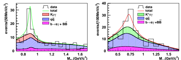
Figure 6. B^+ \rightarrow K^{*0} \pi^+ \gamma and B \rightarrow K^+ \rho^0 \gamma from Belle.
