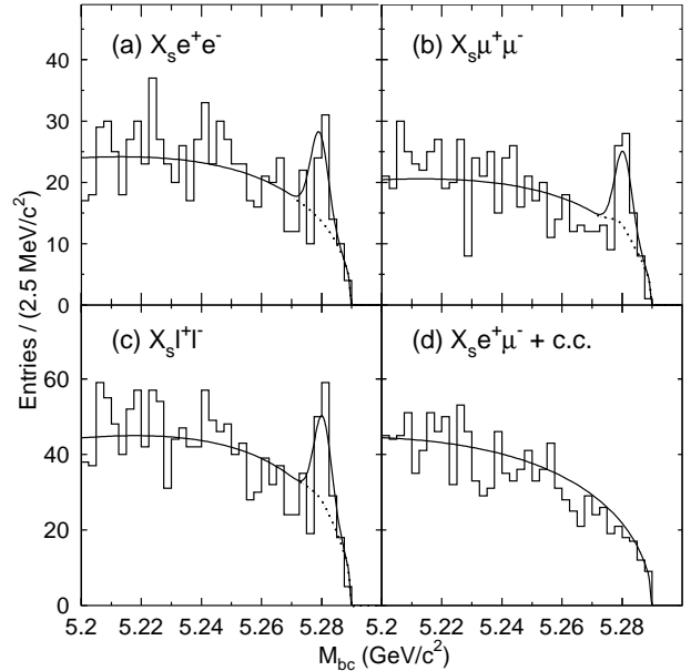
Figure 14. B \rightarrow X_s \ell^+ \ell^- signal measured from Belle. The X_s e^+ \mu^- sample, which is prohibited in the SM, represents the combinatorial backgrounds.
