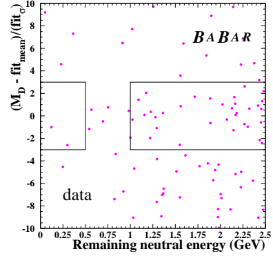
Figure 18. B \rightarrow K \nu \bar{\nu} search results from BaBar using the semi-leptonic tag technique.
