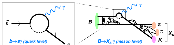
Figure 1. b \rightarrow s\gamma and B \rightarrow X_s\gamma .
