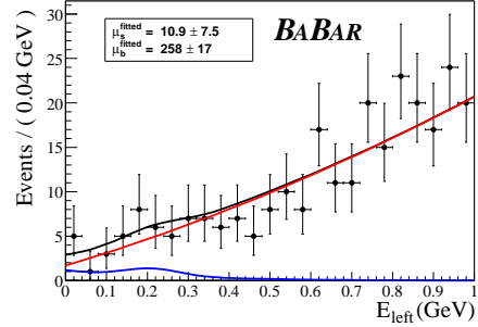
Figure 19. B^+ \rightarrow \tau^+ \nu search results from BaBar using the semi-leptonic tag technique.
