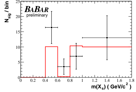
Figure 17. M(X_s) distribution for B \rightarrow X_s \ell^+ \ell^- from BaBar.
