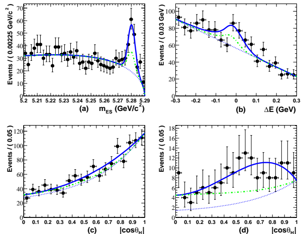
Figure 5. B^0 \rightarrow K_2^*(1400)^0 \gamma signal by BaBar.
