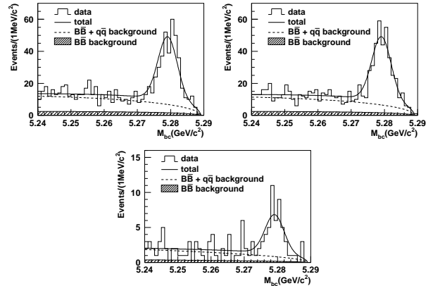
Figure 8. \bar{B} -tagged (top-left), B -tagged (top-right) and ambiguous (bottom) B \rightarrow X_s\gamma signal from Belle.
