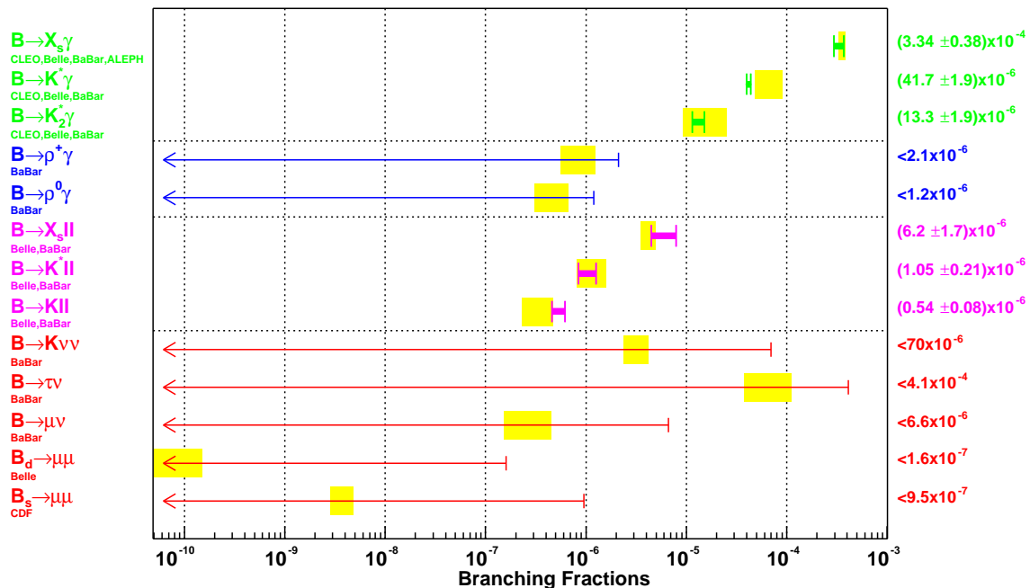
Figure 23. Summary of branching fractions and upper limits compared with the corresponding SM predictions.
