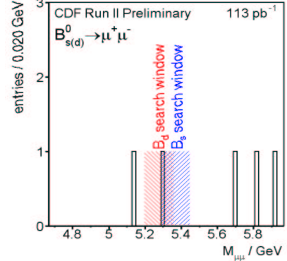
Figure 21. B_s^0 \rightarrow \mu^+\mu^- search results from CDF.
