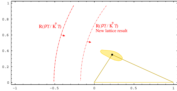
Figure 9. Bound on V_{td} from the ratio of branching fractions of B \rightarrow \rho\gamma to B \rightarrow K^*\gamma .
