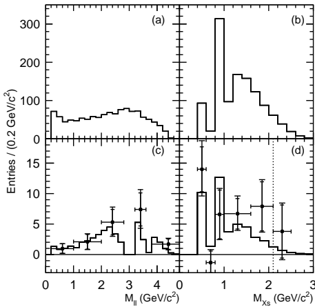
Figure 16. M(\ell^+ \ell^-) (left) and M(X_s) (right) distributions for B \rightarrow X_s \ell^+ \ell^- from Belle (points with error bars), compared with the SM predictions before (top) and after (bottom) including detector acceptance effects.
