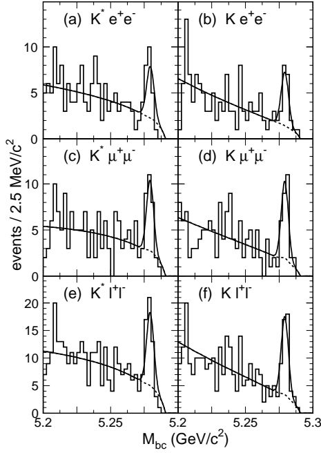
Figure 10. B \rightarrow K^{(*)}\ell^+\ell^- signal observed by Belle.
