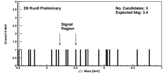
Figure 22. B_s^0 \rightarrow \mu^+\mu^- search results from D0.
