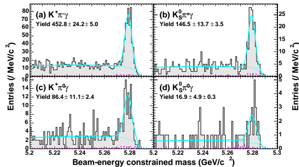
Figure 4. B \rightarrow K^* \gamma signal from Belle.
