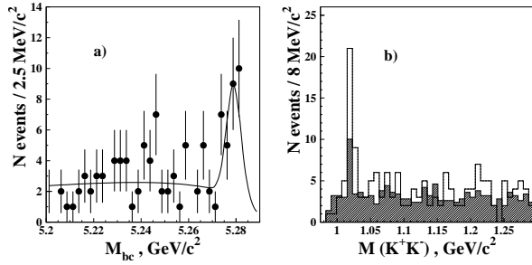
Figure 7. B^+ \rightarrow K\phi\gamma from Belle.
