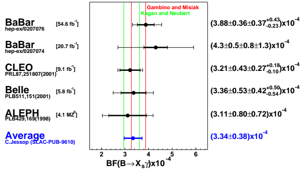
Figure 3. B \rightarrow X_s \gamma branching fraction measurements.
