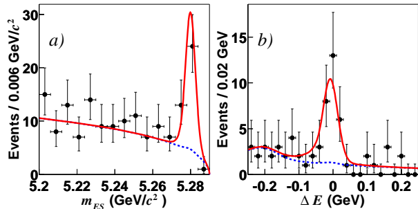
Figure 12. Signal for B \rightarrow K\ell^+\ell^- from BaBar.
