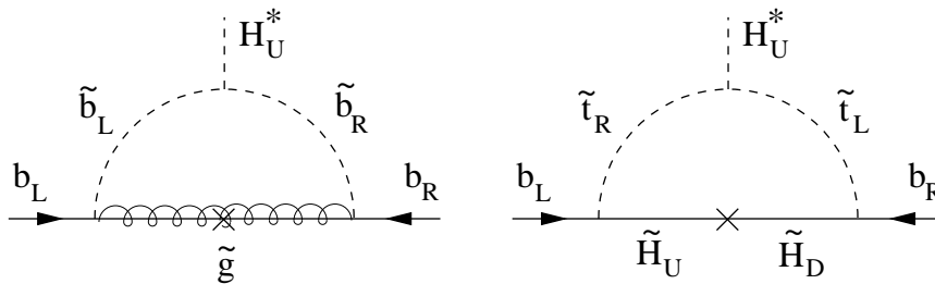
Figure 12: Loop contributions to \Delta\lambda_b .
