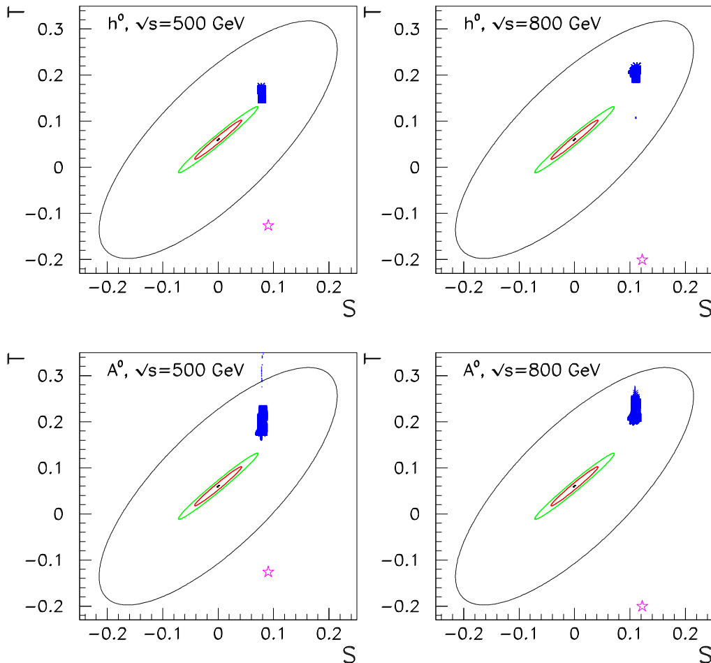
Figure 5: Outer ellipses = current 90% CL region for U = 0 and m_{h_{\text{SM}}} = 115 GeV. Blobs = S, T predictions for Yukawa-wedge 2HDM models with minimum relative \Delta\chi^2 . Innermost (middle) ellipse = 90% (99.9%) CL region for m_{h_{\text{SM}}} = 115 GeV after Giga- Z and a \Delta m_W \lesssim 6 MeV threshold scan measurement. Stars = SM S, T prediction if m_{h_{\text{SM}}} = 500 or 800 GeV.
