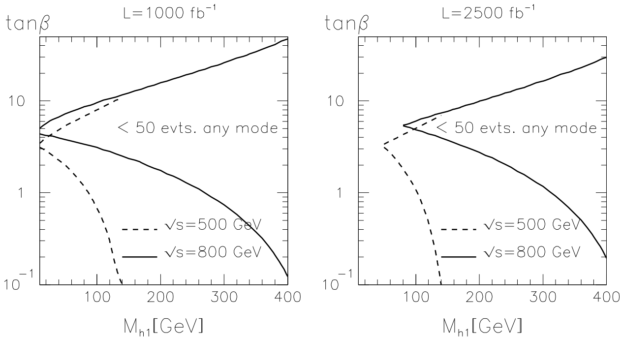
Figure 1: For \sqrt{s} = 500 GeV (dashes) and \sqrt{s} = 800 GeV (solid) the maximum and minimum \tan\beta values between which t\bar{t}h and b\bar{b}h final states both have fewer than 50 events for decoupled h (a) L = 1000 \text{ fb}^{-1} or (b) L = 2500 \text{ fb}^{-1} .
