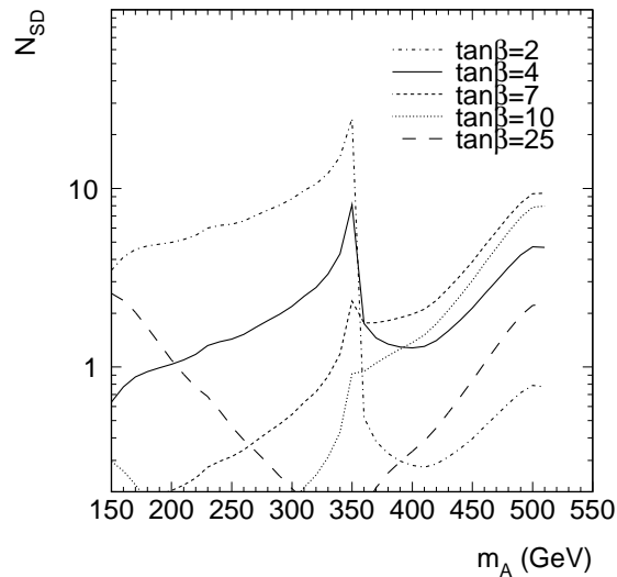
Figure 4: Assuming CAIN 1 year spectra (Fig. 3), we plot the statistical significance of the A^0 signals for a 6 GeV b\bar{b} mass bin centered on m_{A^0} . In (a) [(b)] we employ the case (I) [(II)] spectrum. Various cuts are performed to reduce the background. Efficiency factors other than those coming from kinematic cuts are not included. Resolved photon backgrounds are neglected.
