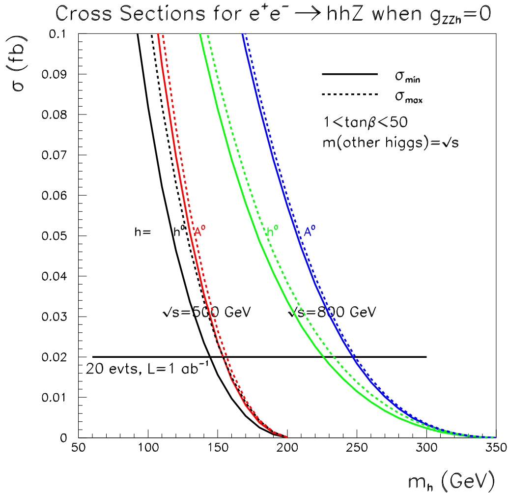
Figure 2: For \sqrt{s} = 500 GeV and 800 GeV and for \hat{h} = h^0 and \hat{h} = A^0 , we plot as a function of m_{\hat{h}} the maximum and minimum values of \sigma(e^+e^- \rightarrow \hat{h}\hat{h}Z) found after scanning 1 < \tan\beta < 50 taking all other Higgs masses equal to \sqrt{s} . For \hat{h} = h^0 , we require \sin(\beta - \alpha) = 0 during the scan. The 20 event level for L = 1 \text{ ab}^{-1} is indicated.
