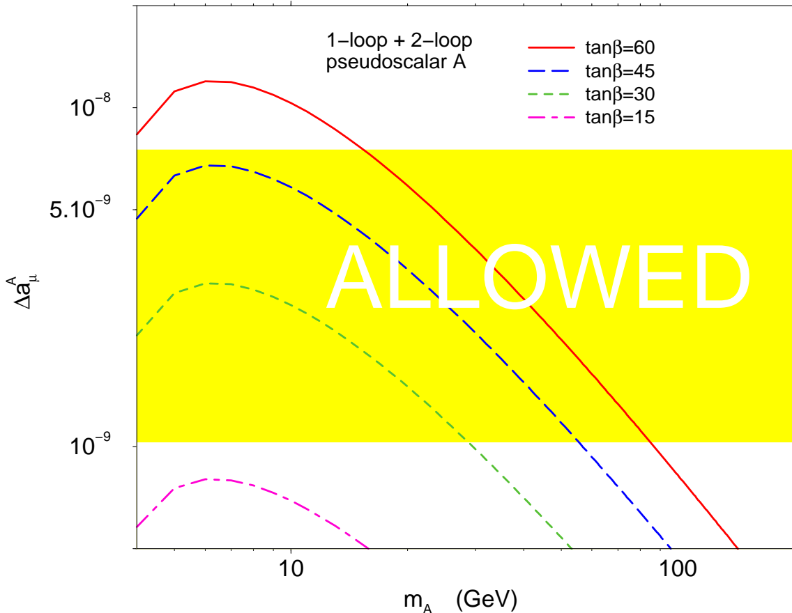
Figure 6: Explanation of new BNL a_\mu value via light 2HDM A^0 . (Cheung, Chou, Kong) In the indicated range of \tan \beta > 17 , it will be found at LC for sure.
