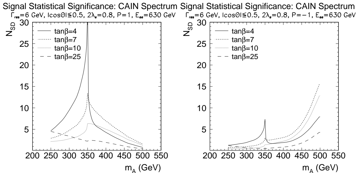
Figure 11: As for A^0 only, but combining H^0 and A^0 signals for maximal mixing case.
