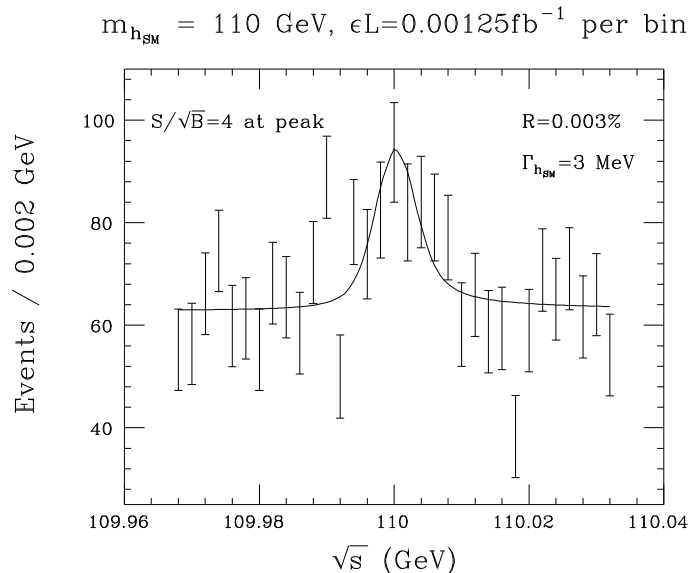
Figure 14: Initial scan for centering on m_{h_{\text{SM}}} = 110 \text{ GeV} Higgs boson.
