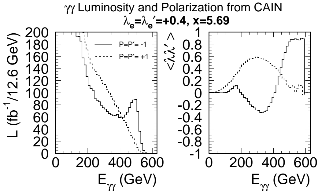
Figure 3: Yearly luminosity in units \text{fb}^{-1}/12.6 \text{ GeV} and associated \langle \lambda \lambda' \rangle are plotted for \sqrt{s} = 630 \text{ GeV} ( x = 5.69 for 1.054 \mu\text{m} laser wavelength), assuming 80% electron beam polarizations, for polarization orientation cases (I) and (II).
