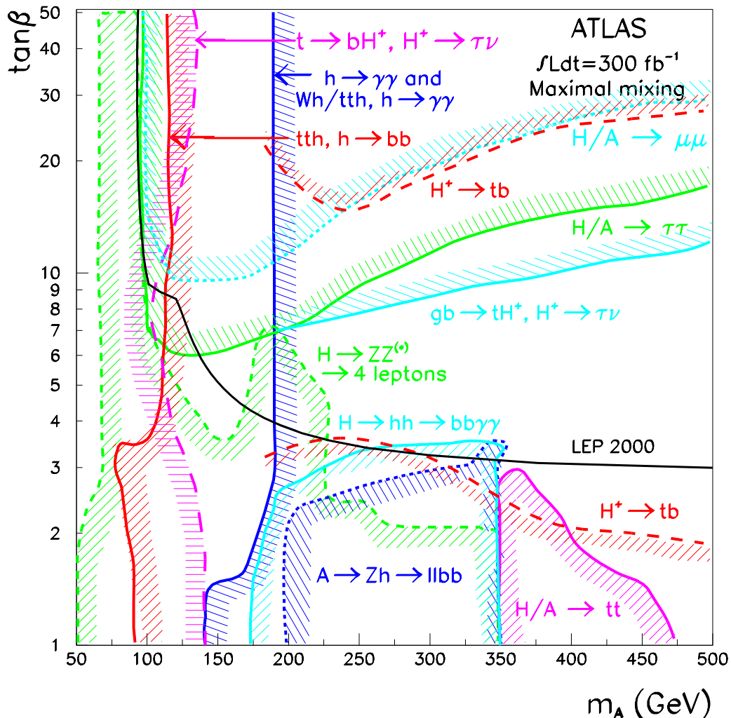
Figure 9: 5\sigma discovery contours for MSSM Higgs boson detection in various channels are shown in the [m_{A^0}, \tan \beta] parameter plane, assuming maximal mixing and an integrated luminosity of L = 300 \text{ fb}^{-1} for the ATLAS detector. This figure is preliminary.
