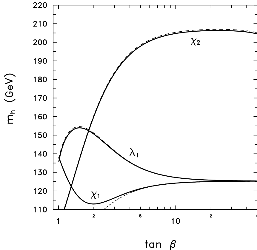
Figure 7: Bounds on SUSY m_h in presence of different types of multiplets. From Espinosa and Quiros, hep-ph/9804235
